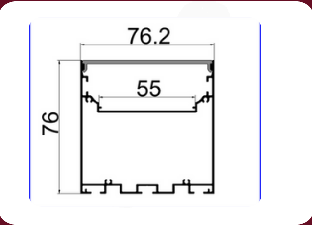
HANGING PROFILE H7575 RECESS MOUNTED 76X76MM ALUMINUM ANODISED PROFILE PC COVER
