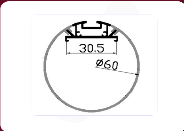
HANGING PROFILE HR60 RECESS MOUNTED DIA.60MM ALUMINUM ANODISED PROFILE PC COVER
