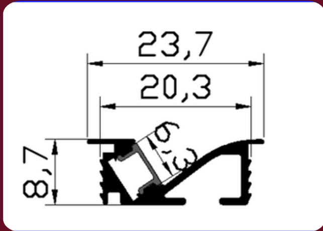
WARDROBE PROFILE W-Z2409
