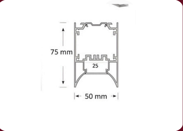
HANGING PROFILE H5075D SURFACE MOUNTED 50X75MM ALUMINUM ANODISED PROFILE PC COVER
