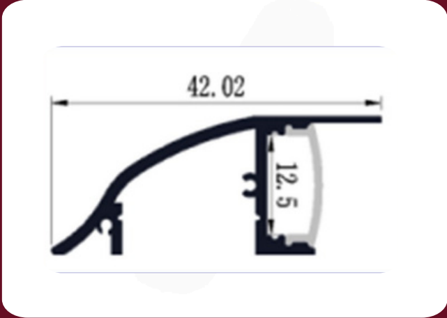
WALL PROFILE W4212 SURFACE MOUNTED 42X12MM ALUMINUM ANODISED PROFILE PC COVER
