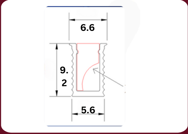
WARDROBE PROFILE W0609
