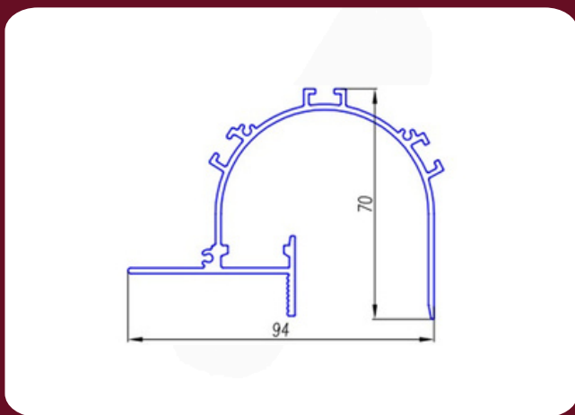
TRIMLESS PROFILE T9470 RECESS MOUNTED 94X70MM ALUMINUM ANODISED PROFILE PC COVER
