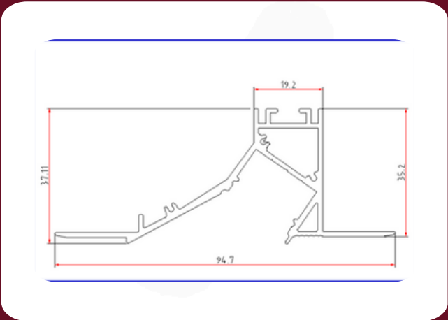
TRIMLESS PROFILE T9535 RECESS MOUNTED 95X35MM ALUMINUM ANODISED PROFILE PC COVER
