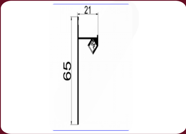
SKIRTING PROFILE SK6521 SURFACE MOUNTED 65X21MM
