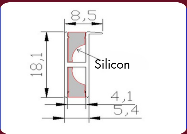
WARDROBE PROFILE S0918
