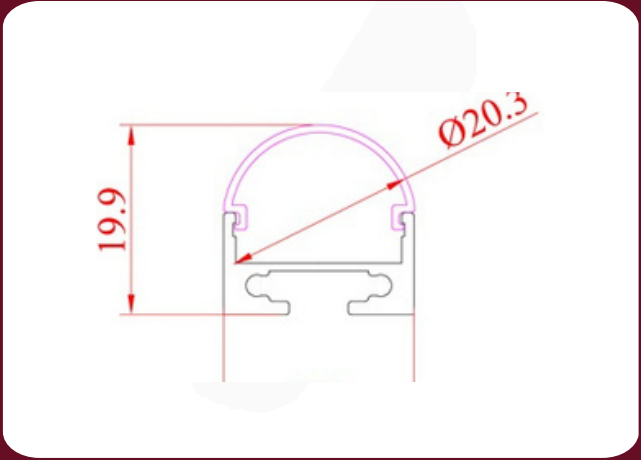
SURFACE PROFILE U2020
