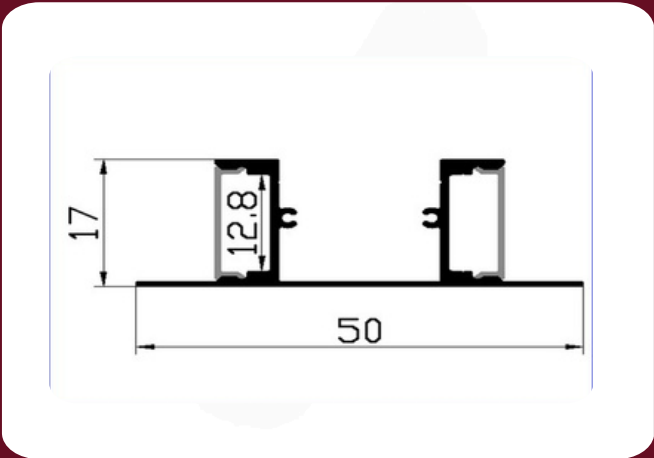
WALL PROFILE R5017 RECESS MOUNTED 50X17MM ALUMINUM ANODISED PROFILE PC COVER
