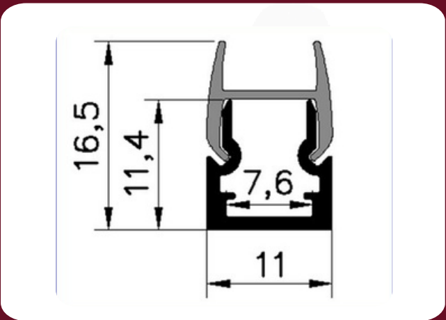
SHELF PROFILE S1117 SURFACE MOUNTED 11X17MM ALUMINUM ANODISED PROFILE PC COVER
