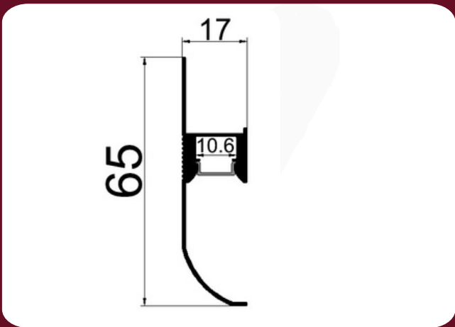
SKIRTING PROFILE SK6517
